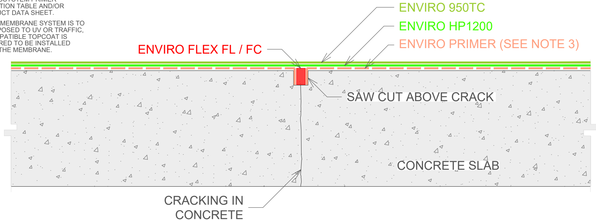
1 WATERPROOFING CRACKING DETAIL SCALE NTS
