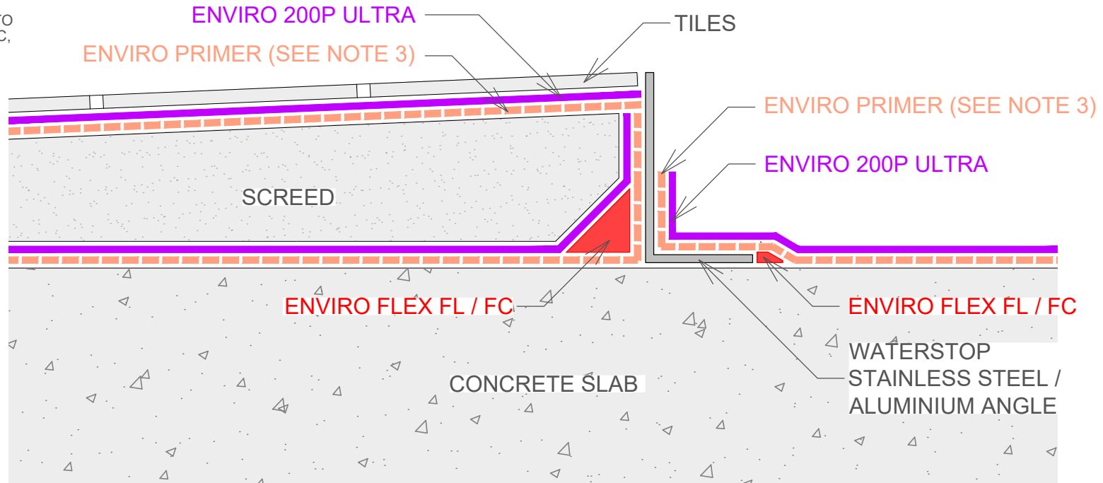
1 ANGLE / WATERSTOP DETAIL SCALE _____ NTS
